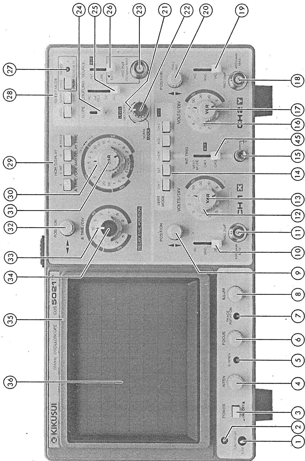
Figure 4-2 (Model COS5021TM)
